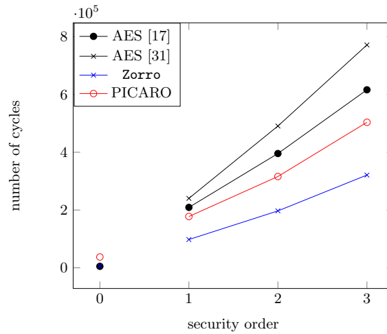
Fig. 4: Performance evaluation.
